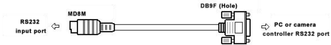
Figure1-6 RS-232 Diagram
